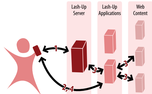
Figure 1. The Lash-Up system interaction for pull-based content. (1) The user accesses the Lash-Up Server to retrieve a list of relevant Lash-Ups. (2) The user chooses an application to access. (3) The application communicates with the Lash-Up Server as well as other web content. (4) The Lash-Up content is delivered to the user.
